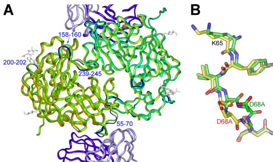
FIGURE 2. Superposition of the structures of the unbound and antibody-bound Bla g 2. A , two monomers of allergen in the unbound state (green) superimposed on the antibody-bound Bla g 2 (yellow and orange). The areas with significant conformational changes are colored blue and labeled. B , area of the largest differences in the vicinity of Asp68a.
